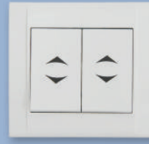
42001026 İKİLİ VAVİEN DOUBLE CUT OUT AND TWO WAY SWITCH Gerilim / Rated Voltage 250V Akım / Rated Current 10A Koruma Derecesi / Protection IP20
